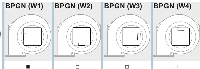
Side assembly, with hole for the power cord
